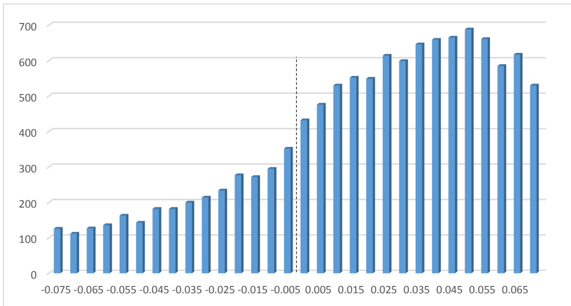
Figure 2. Frequency of observations around zero earnings. Firm-years are grouped into 30 earnings intervals with the width of 0.005 for the range from -0.075 to +0.075.
