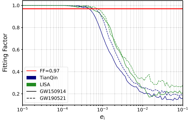
FIG. 2. The fitting factor between a noneccentric template bank and a signal with different eccentricities. The blue (green) lines denote the banks of TianQin (LISA); the solid (dashed) lines correspond to the banks of a GW150914-like (GW190521-like) scenario.
