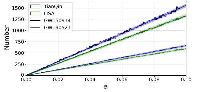
FIG. 3. The distribution of the eccentricity in the archival search template bank. The shaded regions represent the 1\sigma Poisson fluctuation.
