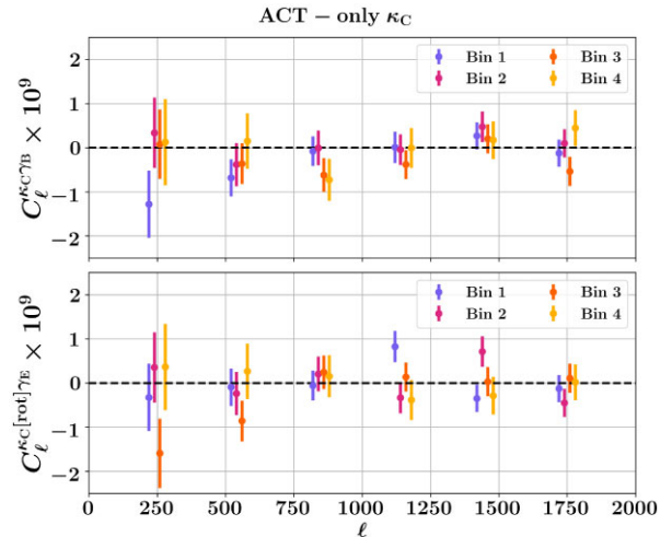
Figure A2. Similar to Fig. 10, but for ACT-only data. Top: The power spectrum between \kappa_C and the B-mode of the shear ( C_\ell^{KCYEB} ), which is expected to be consistent with zero. Bottom: The correlation between \kappa_C and the E-mode of the shear map ( C_\ell^{KCYE[rot]} ) obtained from the catalogue in which ellipticities are randomly rotated.
