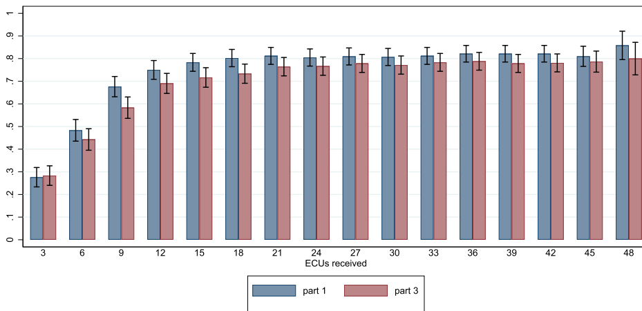
Fig. 5. Probability of being trustworthy. Note: The amount received, displayed on the horizontal axis, is the amount allocated by the trustor multiplied by 3. Capped spikes represent 95% confidence intervals.
