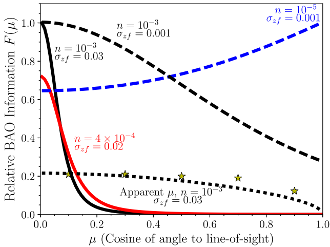
Figure 2. The relative amount of BAO information as a function of \mu , the cosine of the angle to the line of sight, for a sample of galaxies at z = 0.8 , with properties as labelled. We use \sigma_{zf} = \sigma_z/(1+z) and the number density n is in units h^3 \text{Mpc}^{-3} . All cases use a galaxy bias of b = 1.8 , except for the solid red curve, which assumes b = 2 . The dashed curves represent redshift precision achievable from spectroscopic galaxy surveys, while the solid curves show results achievable from multiband imaging surveys, such as the Dark Energy Survey. All results are in terms of the true \mu , except for the dotted curve, which displays the information in terms of observed \mu . Results are normalized as follows: The solid black and red curves and the black dashed curve are all divided by the same factor; thus, they are directly comparable. The blue dashed curve is normalized such that it has the same maximum value as the black dashed curve; it thus illustrates how the relationship between BAO information and \mu changes with number density. The black dotted curve displays the same information as the black solid line, but with respect to observed \mu ; the area under the apparent \mu curve is normalized to be twice that of the solid black curve (for legibility). The yellow stars represent what we find for mock galaxy samples, normalized so that the results match the dotted curve at \mu = 0.1 .
