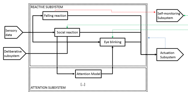
Fig. 11. High level description of the reactive subsystem.
