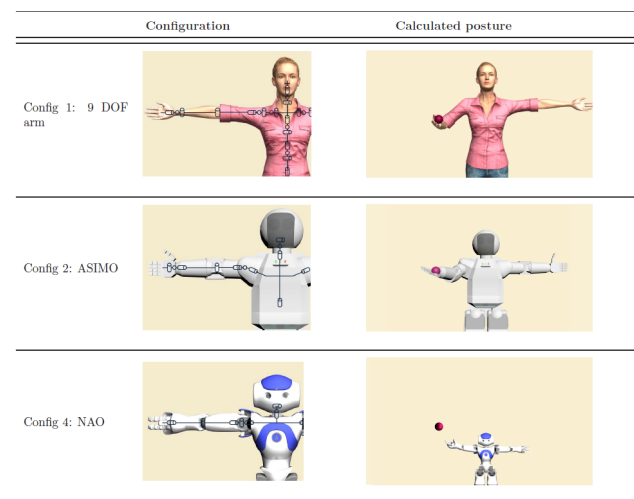
Fig. 14. Results of the method for different arm configurations. The first column shows the joint configuration, while the second column shows the end posture for a place-at gesture at (34, -34, 38) .
