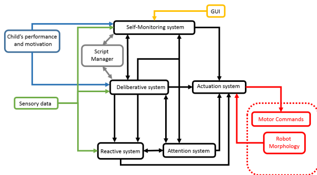
Fig. 10. Description of the cognitive controller subsystems and how information flows from one subsystem to another.
