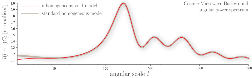
Figure 1. The normalized CMB angular power spectrum, from [72]. The power spectrum is shown against a default flat concordance model with zero tilt. There is nothing between the two models for high \ell , with the maximum difference around 1%.
