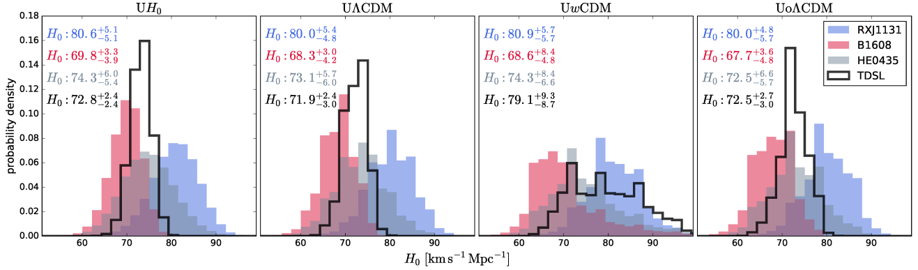
Figure 4. Marginalized posterior probability distributions for H_0 in the UH_0 , U\Lambda CDM, Uw CDM and Uo\Lambda CDM cosmologies using the constraints from the three strong lenses B1608+656, RXJ1131–1231 and HE0435–1223. The overlaid histograms present the distributions for each individual strong lens (ignoring the other two datasets), and the solid black line corresponds to the distribution resulting from the joint inference from all three datasets (TDSL). The quoted values of H_0 in the top-left corner of each panel are the median, 16th and 84th percentiles.
