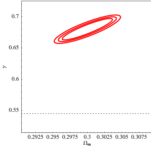
FIG. 12: Confidence regions at 68% for the benchmark survey z_{mean} = 0.9 , d = 35 (outer contour) and for d = 50, 75 (inner contours) for DGP. The dotted line represents the \Lambda CDM value. From [75].
