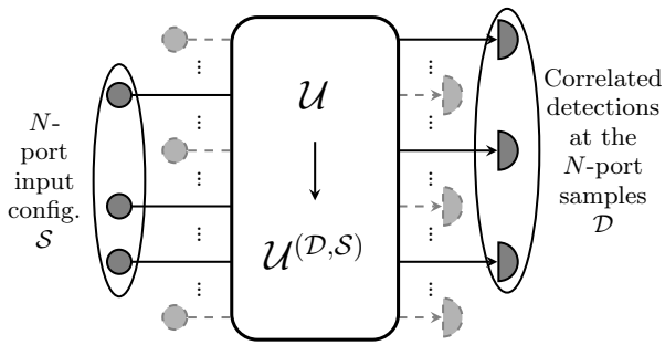
FIG. 1. General setup for multiboson correlation interferometry. N single bosons are injected into an N -port subset \mathcal{S} of the M input ports of a linear interferometer. They can be detected at the output in any possible sample \mathcal{D} containing N of the M output ports at N corresponding detection times \{t_d\}_{d \in \mathcal{D}} . For each output port sample \mathcal{D} and given input configuration \mathcal{S} , the evolution through the interferometer is fully described by a N \times N submatrix \mathcal{U}^{(\mathcal{D}, \mathcal{S})} of the original M \times M interferometer matrix \mathcal{U} . The correlated measurements can be performed in any bosonic degree of freedom, such as time, polarization and spin.
