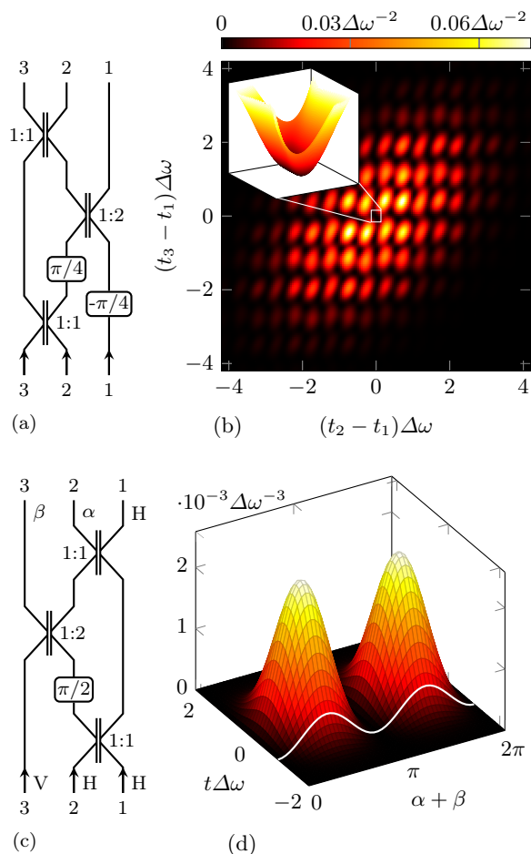
FIG. 2. (Color online) Correlation landscapes at the output of a tritter for three input photons with Gaussian spectra with identical variance \Delta\omega^2 but different central frequencies ( \omega_{0,2} - \omega_{0,1} = 8.0\Delta\omega , \omega_{0,3} - \omega_{0,1} = 12.7\Delta\omega ). In panel (b), we observe three-photon quantum beats in the threefold coincidence rate measured at the output of the tritter in panel (a) for equally polarized input photons and polarization-independent detections. The inset magnifies the three-dimensional “dip” occurring at equal detection times. In panel (c), H -, H -, and V -polarized input photons impinge on a symmetric tritter. The emergence of W -state-type correlations for joint detections at approximately equal times t is shown in panel (d) (here, for simplicity, the propagation time is \Delta t \cong 0 ): if a H -polarized photon is detected in one output port we observe in the remaining two ports 100% visibility correlations in the sum \alpha + \beta of the detected polarization angles typical of a Bell state (indicated for an arbitrary time t by the white curve).
