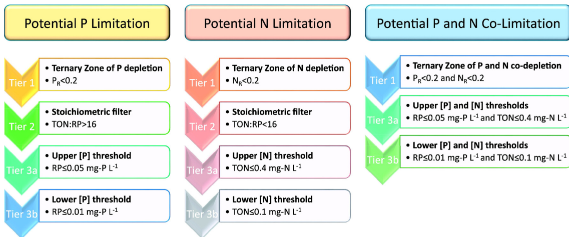
Fig. 3. Nutrient Limitation Assessment framework, showing the P and N criteria for the sequential tiers of assessment of potential P and N limitation and co-limitation.
