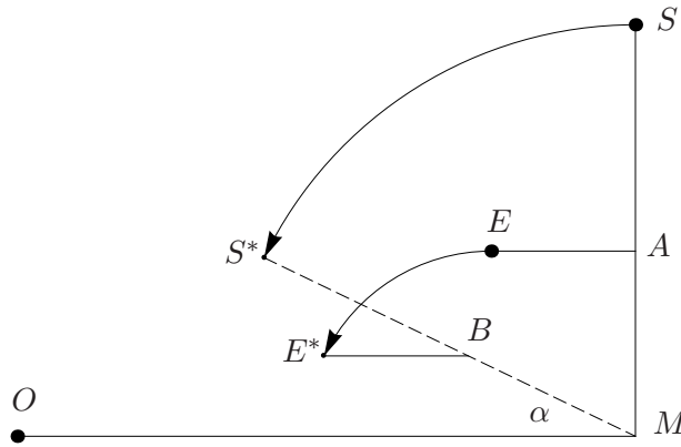
FIGURE 4. An east-growing ray starts at O and a south-growing ray starts at S . In the absence of other rays, their paths in the \alpha = 90^\circ case would meet at M . When \alpha is changed to the value shown in the figure, consider what happens if S is moved around the circular arc to S^* before ray growth commences. The ray then grows from S^* toward M . Because the arc has centre M , |S^*M| equals |SM| , and because O is (0,0) and M is fixed, |OM| is unchanged. So we see that (in the event that ray S and ray O actually reach M ) which one blocks the other is unchanged. At E , however, is another east-growing ray; obviously it might block S (at A ). The role of this third ray, and any other relevant rays, is discussed further in the text.
