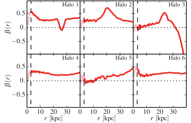
Figure 8. Stellar anisotropy profile \beta(r) as a function of radius for the six EAGLE clusters over the radial range relevant to the stellar kinematics analysis. The vertical dashed line on each panel shows the 3D convergence radius, r_c and the profiles at lower radii are shown using shaded lines. Two BCGs are consistent with \beta = 0 but would be better fit with a non-constant \beta . Ignoring complex features, the other four clusters present more radially biased orbits with \beta(r) \approx 0.25 . A single profile shape for \beta(r) cannot be used to characterize all six of our BCGs.
