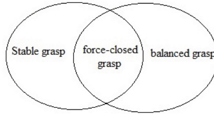
Figure 1. Relationship of stable, balanced and force-closed grasp
