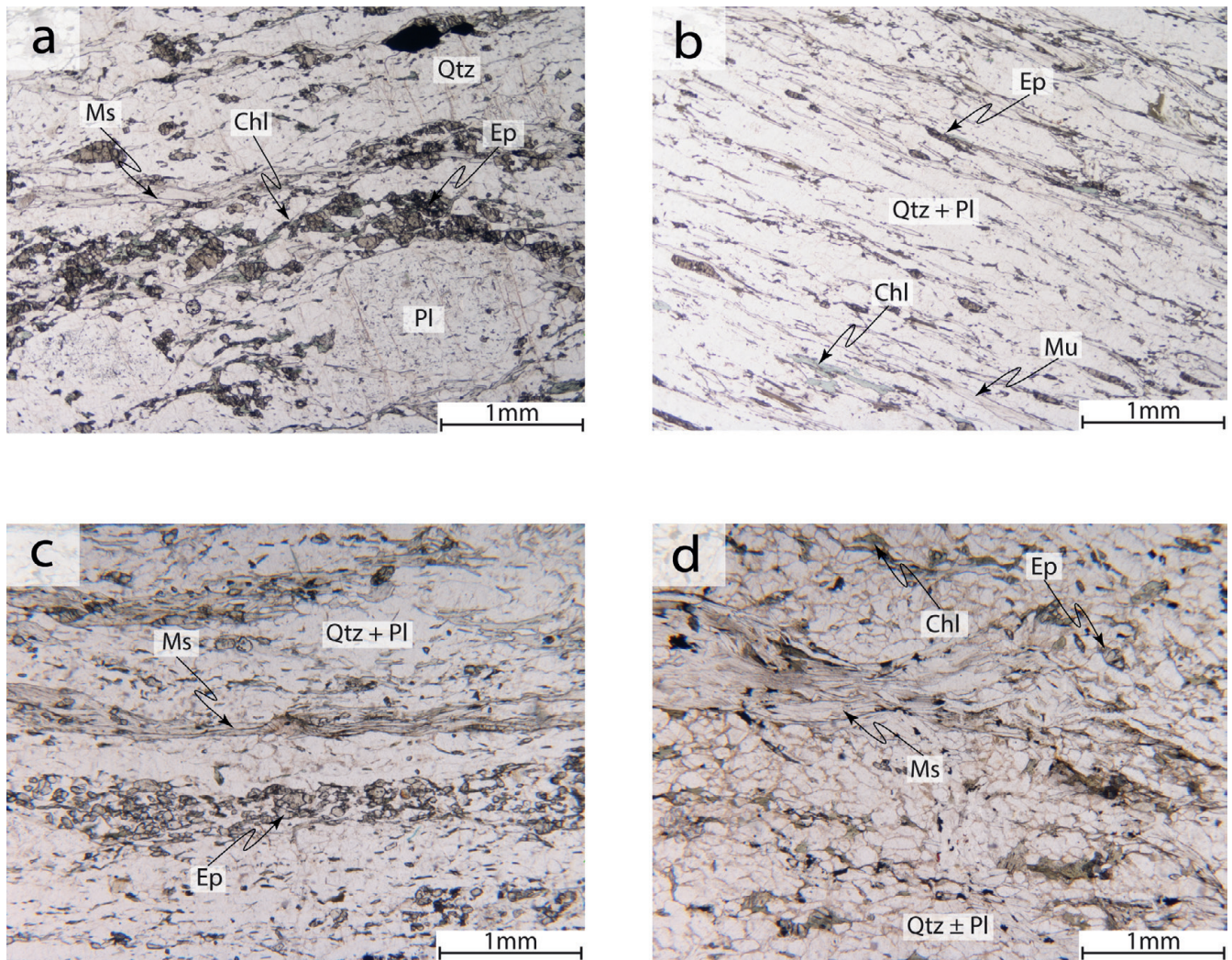
Fig. 7. Thin section photomicrographs in plane-polarized light from North Roe: (a) SW12-01; (b) SW12-02; (c) SW13-01; (d) SW13-03. Mineral name abbreviations taken from Kretz (1983).
