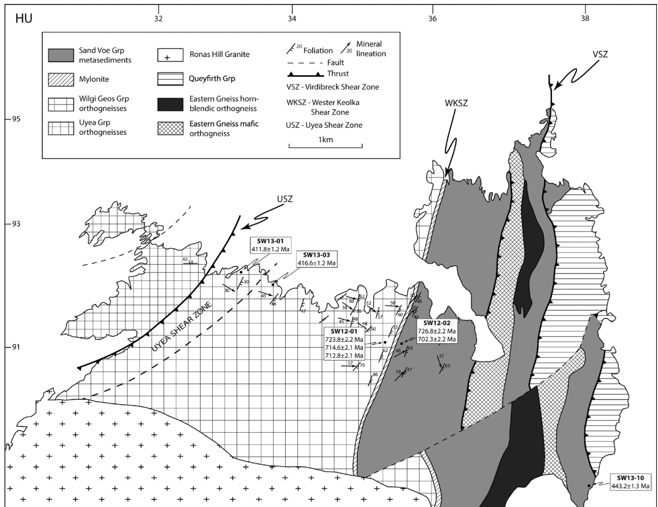
Fig. 2. Geology of the North Roe region of northern Mainland Shetland, including sample sites and age determinations.
