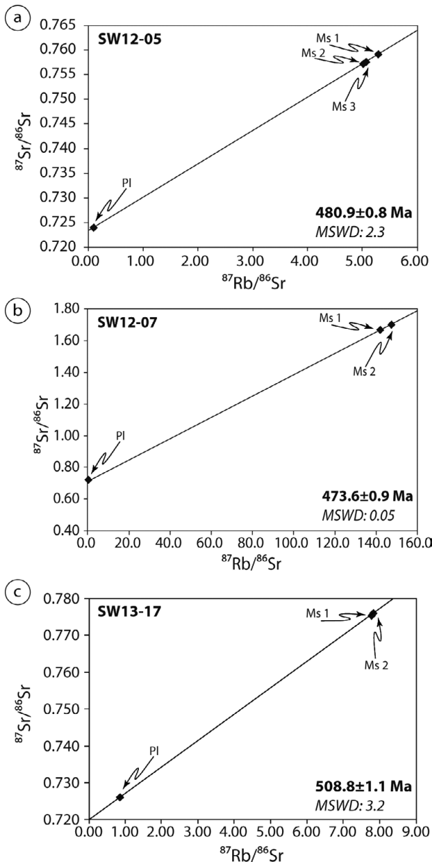
Fig. 5. Rb–Sr isochron diagrams for samples where multiple mica separates were analysed. Pl, plagioclase fraction; Ms, white mica, with fraction indicated numerically. Error bars are smaller than symbols.
