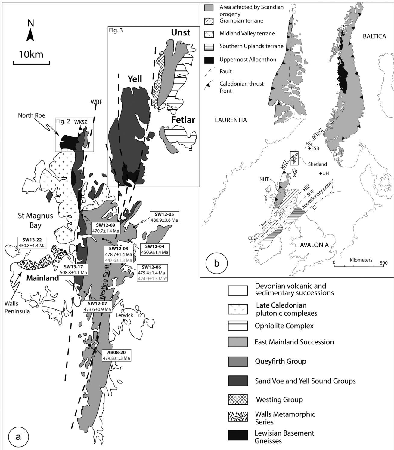
Fig. 1. (a) Simplified geological map of Shetland including sample sites on Mainland. (b) Regional context of Shetland in its pre-Mesozoic rifting setting (modified from Bird et al. 2013). Ages shown in grey are biotite–feldspar ages; all others are white mica–feldspar. WBF, Walls Boundary Fault; WKSZ, Wester Keolka Shear Zone; IS, Iapetus Suture; SUF, Southern Uplands Fault; HBF, Highland Boundary Fault; GGF, Great Glen Fault; MTZ, Moine Thrust Zone; NHT, Northern Highland Terrane; MTrFZ, Møre–Trøndelag Fault Zone; ESB, East Shetland Basin; UH, Utsira High; CB, Clew Bay. Asterisk indicates ages that are not robust.
