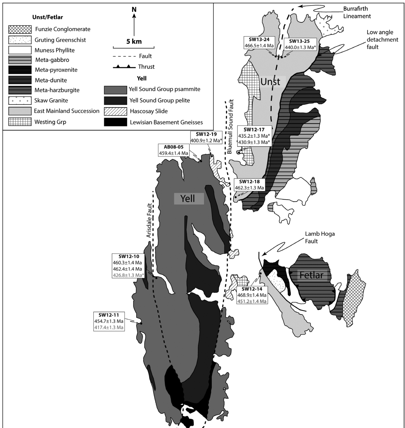
Fig. 3. Geology of the islands of Yell, Unst and Fetlar in Shetland, including sample sites and age determinations. Ages shown in grey are biotite–feldspar ages; all others are of white mica. Asterisk indicates ages that are not robust.
