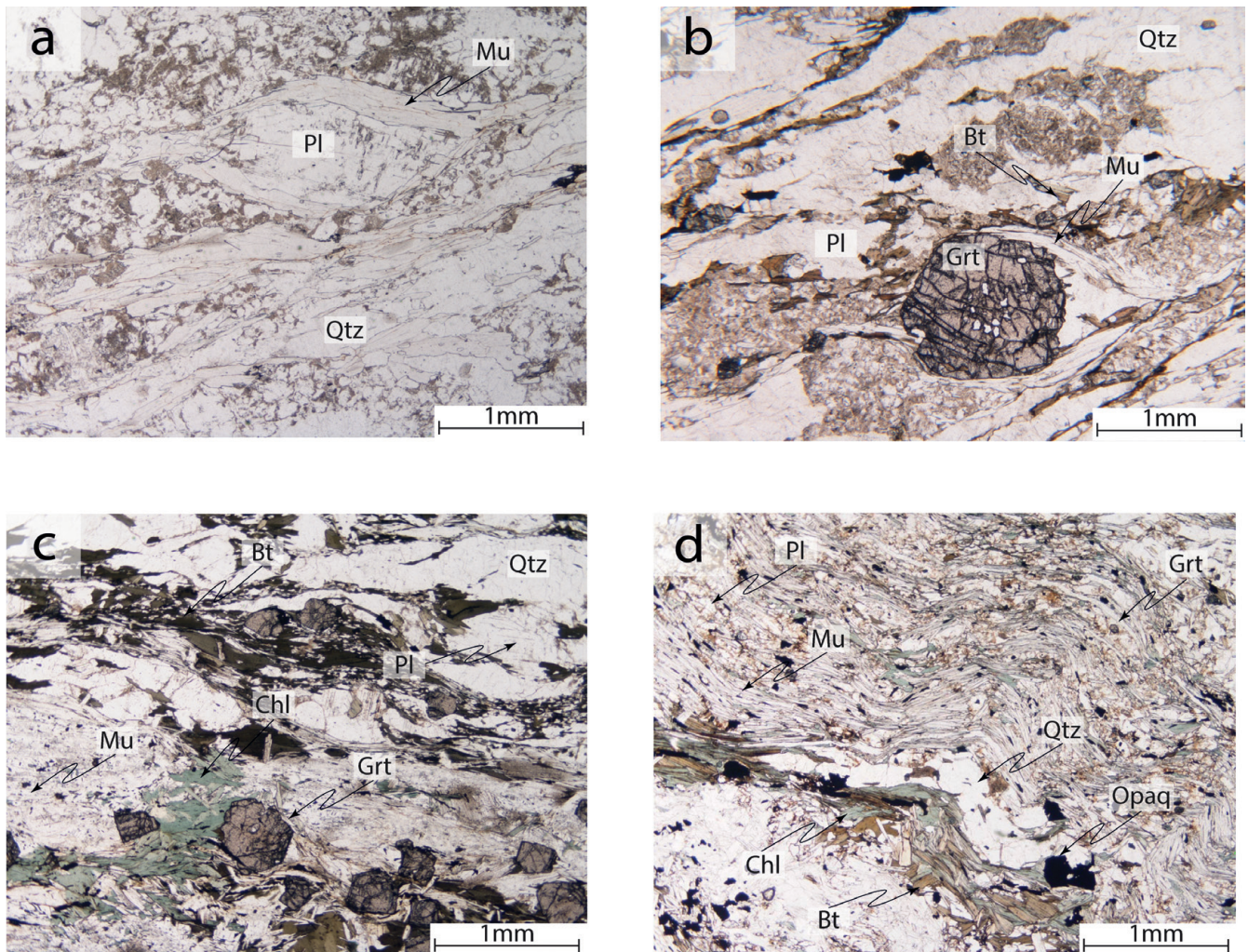
Fig. 6. Representative thin section photomicrographs in plane-polarized light: (a) SW12-07; (b) SW13-17; (c) SW12-14; (d) SW13-25. Mineral name abbreviations taken from Kretz (1983).
