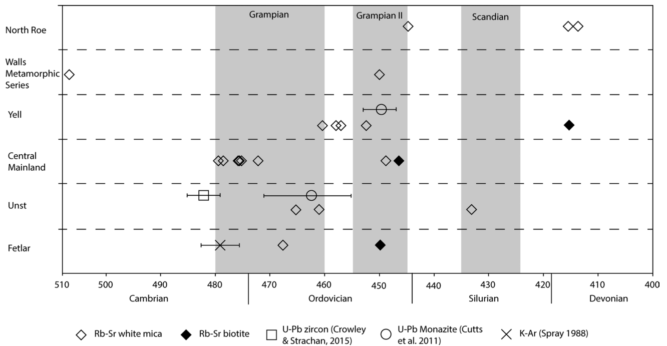
Fig. 4. Graphical representation of Caledonian ages in Shetland, including data from this study and other modern geochronological work. For ages where no error bars are shown, uncertainties are smaller than the marker symbol.
