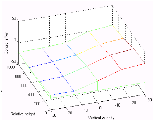
Figure 5: Output surface for the compressed system
