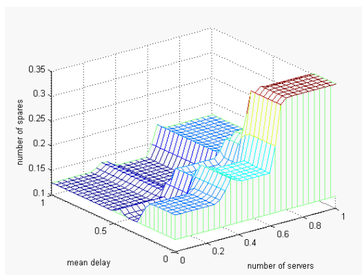
Figure 15: Output surface for the compressed system with input 1 = 0
