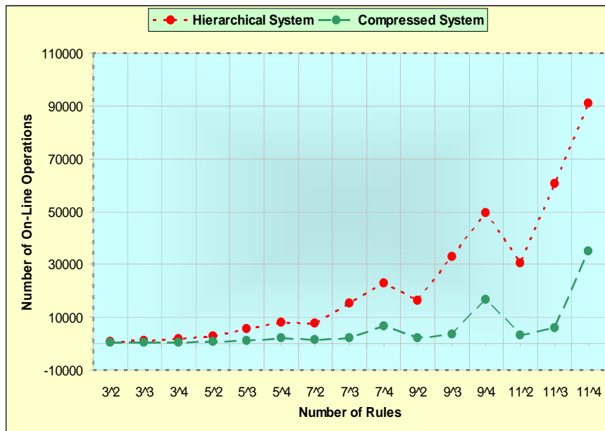
Figure 20: Complexity of the hierarchical and the compressed system
