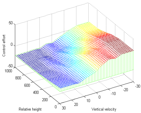
Figure 12: Output surface for the original system
