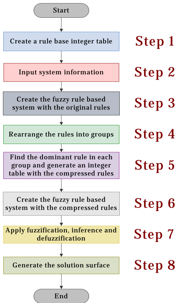
Figure 3: Algorithm for rule base compression
