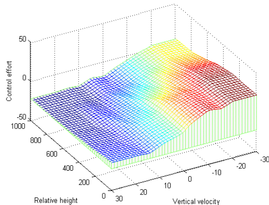
Figure 13: Output surface for the compressed system
