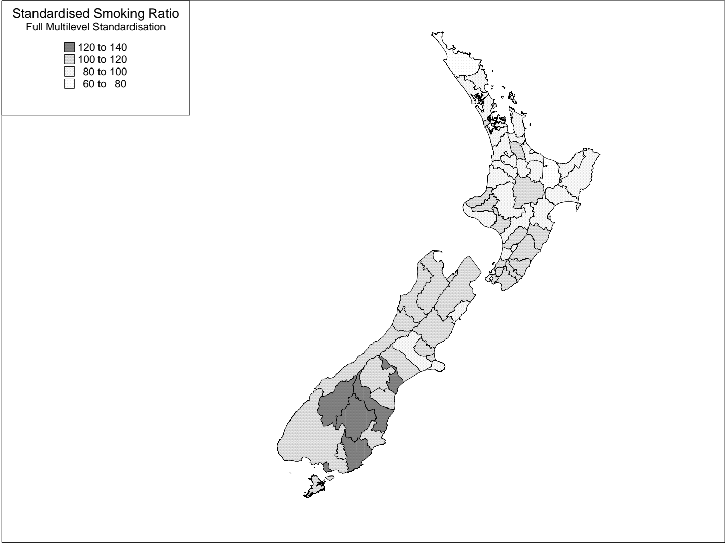
Figure 2: Residuals from Full Multilevel Analysis
