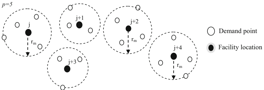
Fig. 9 The case where (s+1) facilities have the same maximum distance ( r_m )
