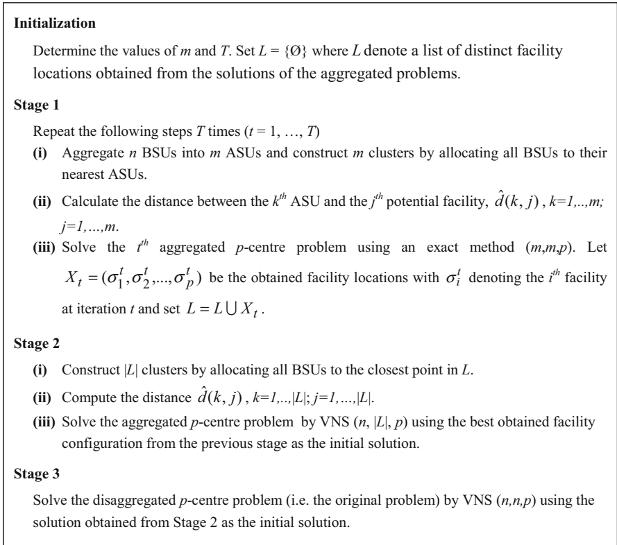
Fig. 1 The main steps of the Three-stage Approach (TSA)
