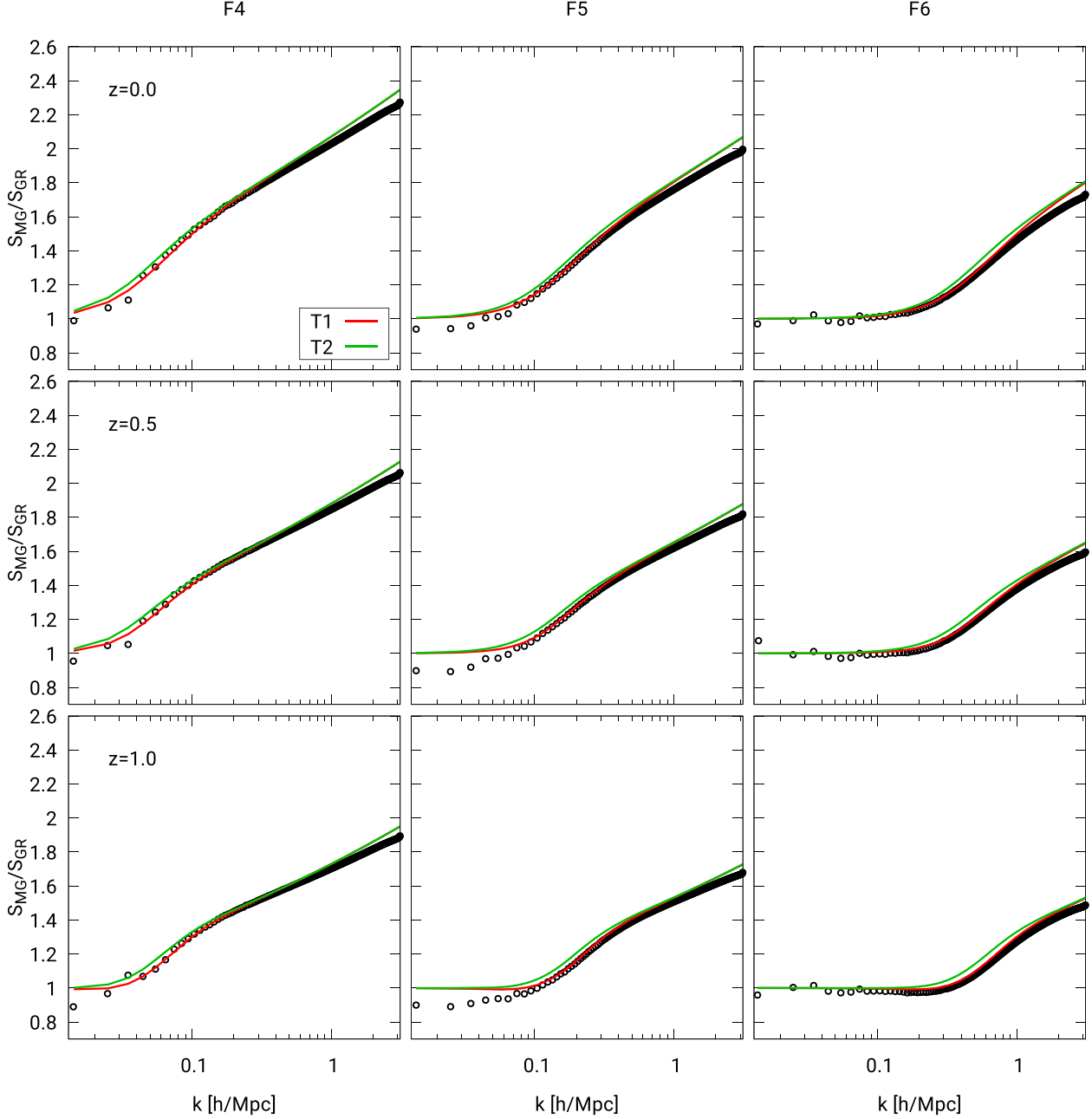
Figure 4. Computation of the full source term (black dots), compared to the triangle configurations T1 (orthogonal: k_1 = k_2, \theta = 90^\circ , red line) and T2 ( k_1 = k_2, \theta = 80^\circ , green line), for different redshifts and different values of the f_{R0} parameter. Top row is z = 0 , middle row z = 0.5 , and bottom row is for z = 1 . The left column is f_{R0} = -10^{-4} , middle column f_{R0} = -10^{-5} , and right column f_{R0} = -10^{-6} . For each redshift and each value of f_{R0} , we compute the source term for a box with 700^3 particles and L = 700 \text{ Mpc } h^{-1} .
