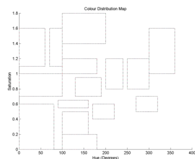
Figure 9: HSB Colour Distribution
