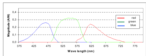
Figure 8: MCS Sensitivity.
