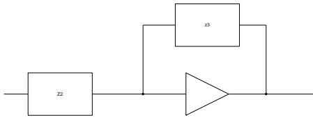
Figure 10: High Pass Filter
