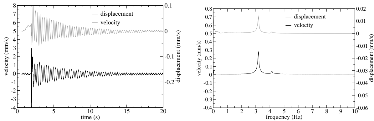
Figure 13. Free vibration of the model silo containing PET pellets.
