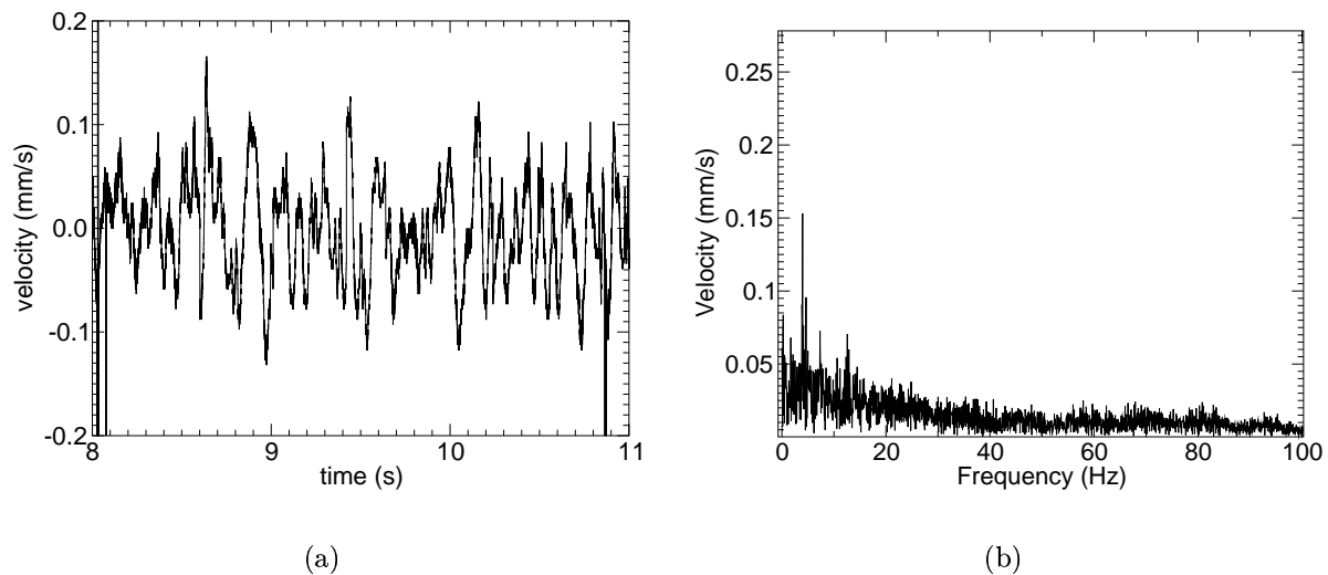
Figure 12. Velocity measurements during discharge of barley: typical velocity variation with (a) time and (b) frequency.
