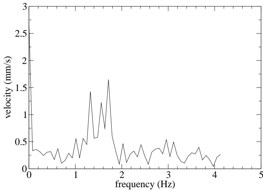
Figure 6. Velocity spectrum during discharge of PET pellets.
