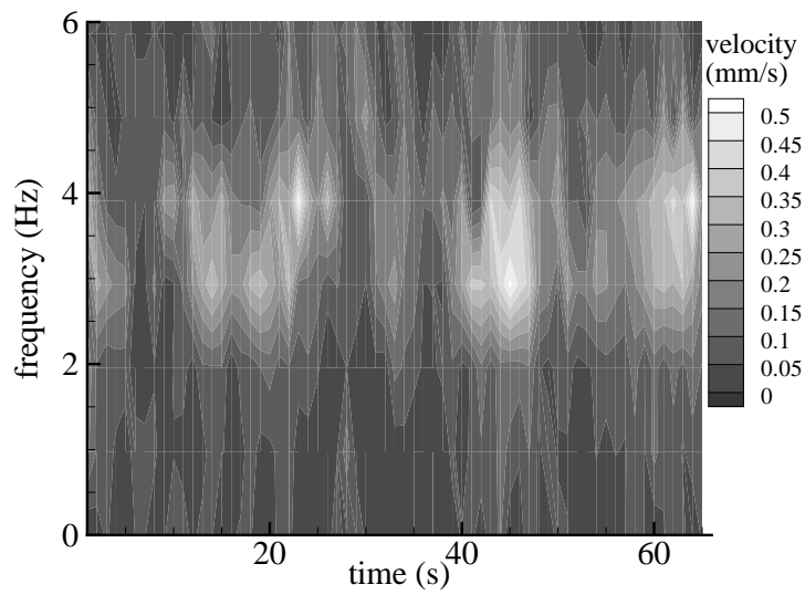
Figure 11. The frequency spectrum as a function of time.
