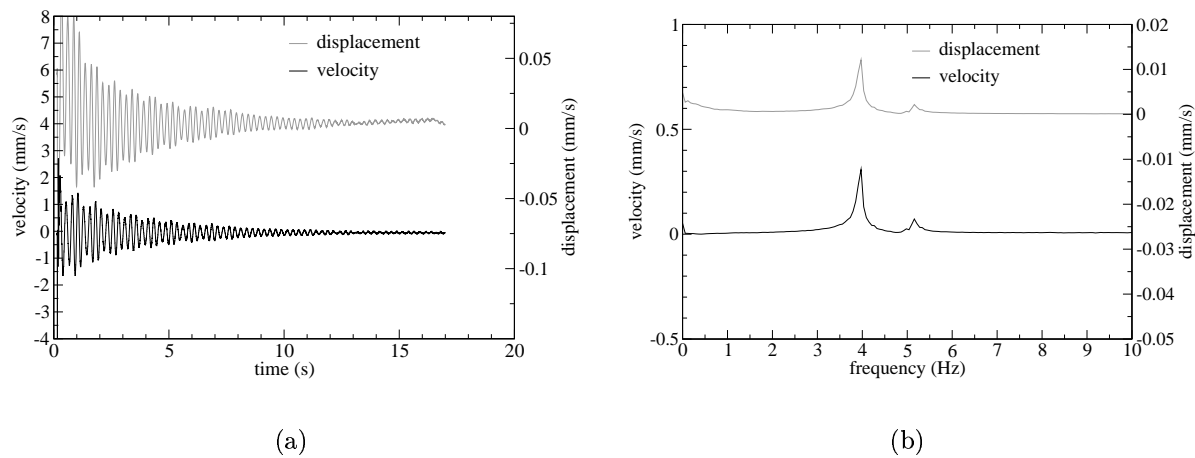
Figure 14. Free vibration of the model silo containing barley.
