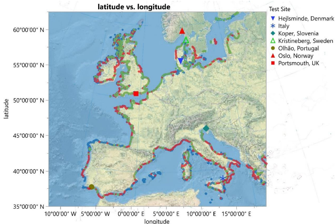
Fig. 2: Permanent marine test sites for wood treatments and overview of coastal erosion patterns in Europe according to the European Environment Agency (2016); (aggradation in green, erosion in red, stable conditions in blue)
