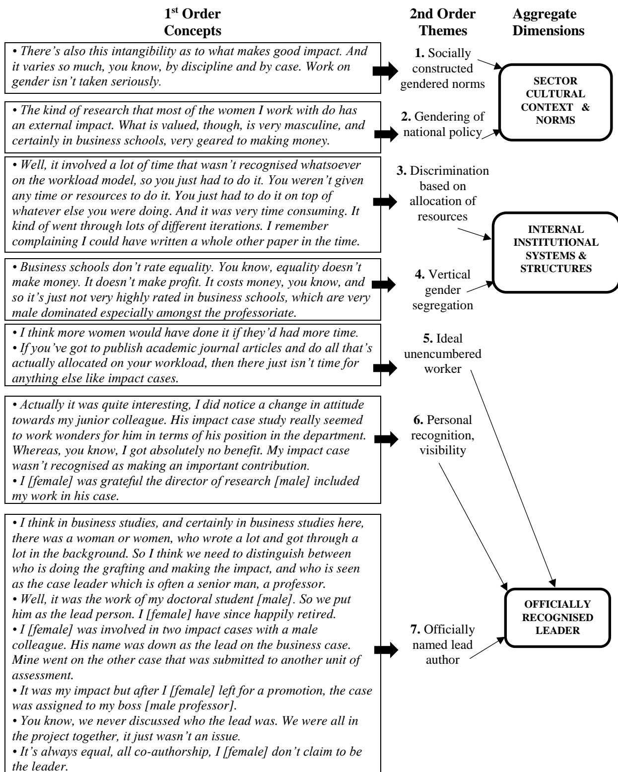
Figure 1: Data structure
