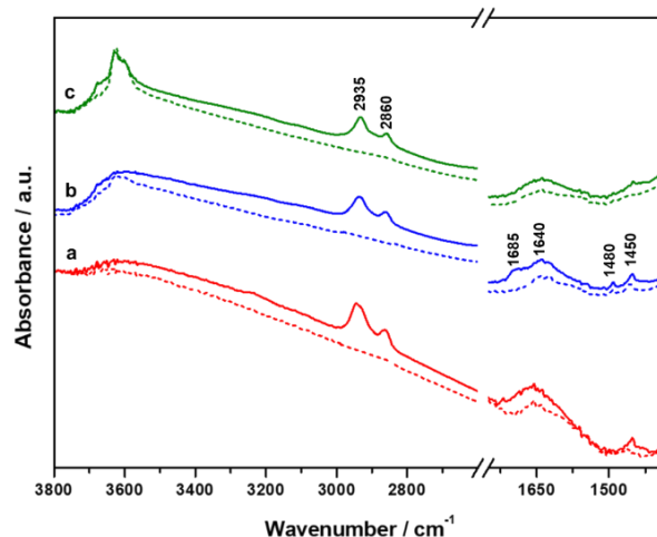
Figure 6. The FT-IR spectra of HP AIPO-5 (curve a, red), HP SAPO-34 (curve b, blue) and SAPO-34 (curve c, green) before (dotted lines) and after (solid lines) exposure to cyclohexanone oxime, at room temperature.
