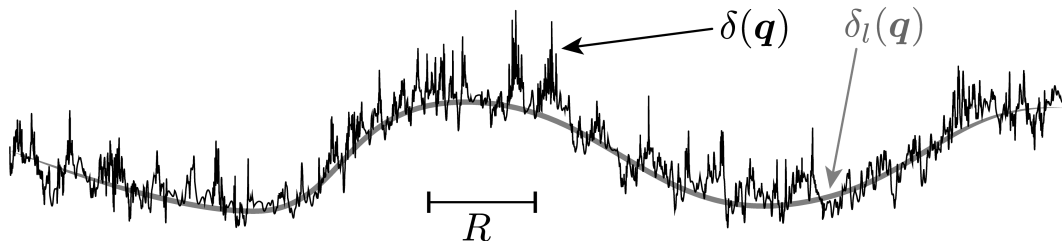
FIG. 2. The thick grey line is the long mode of the dark matter density field, while the snaky black line is the total dark matter density fluctuation. The short modes are responsible for the intrinsic scatter around \delta_l .
