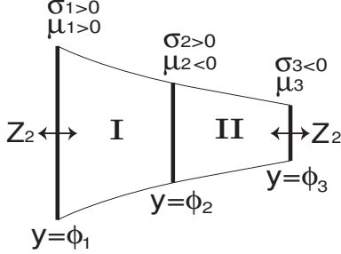
FIG. 6: three-brane system
