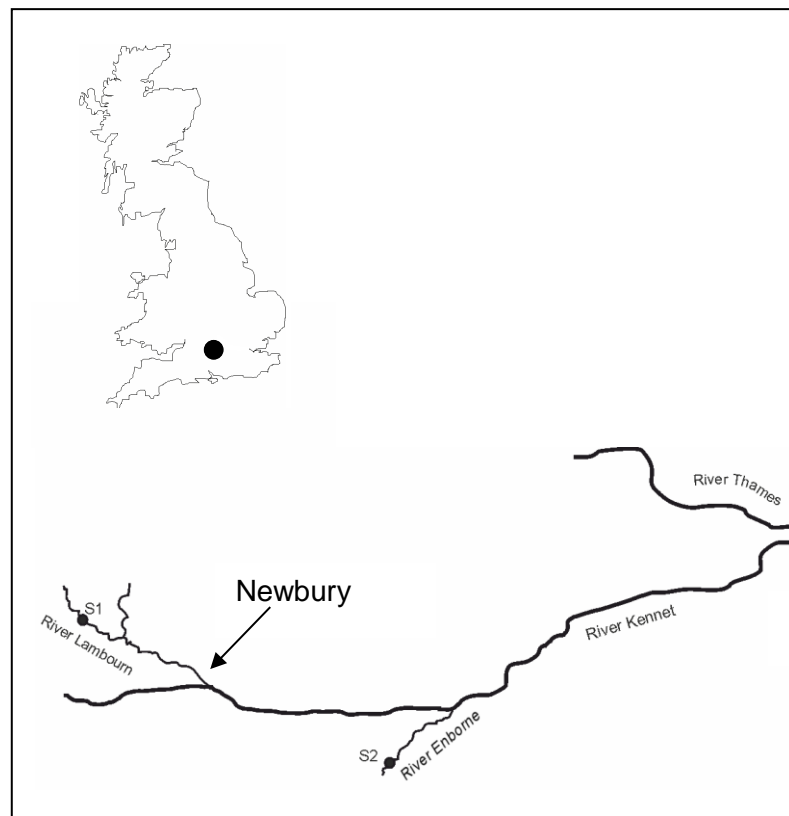
Fig. 1 Location of field sites in the UK. Site 1 (S1) is located on the River Lambourn and site 2 (S2) on the River Enborne. Both rivers are tributaries of the River Kennet within the River Thames catchment.
