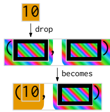
Fig. 10. Using the tuple construction (comma) operator block
