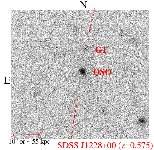
Figure 18. Narrow band continuum image of the field around SDSS J1228+00. It was obtained with the H\alpha+83 FORS2 filter and covers the rest frame spectral range \sim 4150-4185 Å. The PA 170 slit location is indicated. G1 is a continuum source of unknown z .
