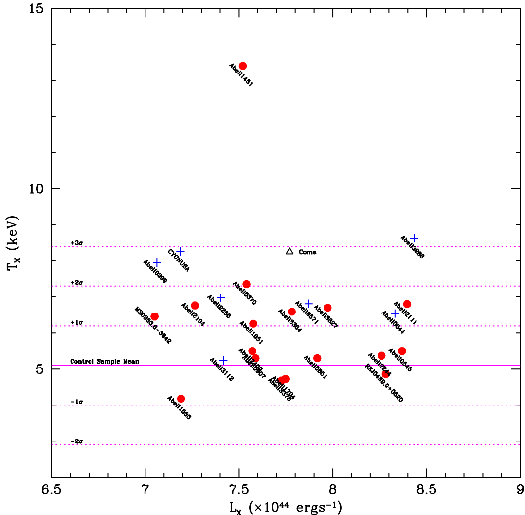
Figure 1. X-ray temperatures for clusters extracted from BAX within 1 \times 10^{44} erg s ^{-1} of Coma’s X-ray luminosity that have T_X values available. Clusters below z = 0.0814 are marked with blue pluses, those above with red filled circles. Coma is marked by a triangle near the centre of the plot. The mean T_X of our control sample (i.e. those clusters inside the SDSS boundary that are within 5 \times 10^{44} erg s ^{-1} of Coma’s X-ray luminosity) is denoted by the solid horizontal line and a few standard deviations either side of this are represented by the dotted lines, as labelled. Coma has one of the largest T_X values for this narrow L_X range and is \sim 2.9\sigma above the control sample’s mean T_X value.
