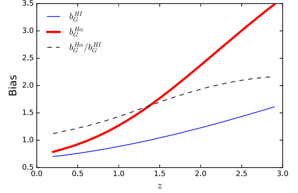
Figure 1. Gaussian bias of \text{HI} (thin solid blue Santos et al. 2015) and \text{H}\alpha (thick solid red; Fonseca et al. 2017b) emission lines. The ratio of the biases is also shown (dashed).
